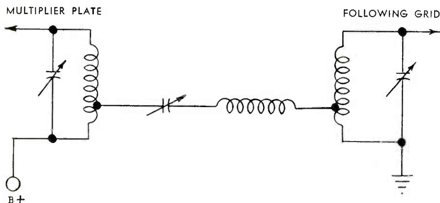
FIGURE 1 PHASE LINEAR MULTIPLIER COUPLING
